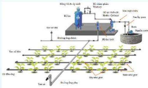
Pumping and drip irrigation system
