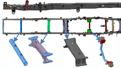
Chassis
